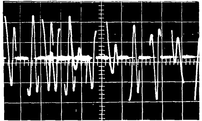
FIGURE 9. Wave Form at Demodulator Shown with Some Pickup. Measurements are adequate; there is no offset but some noise. Scale is 0.5 v/cm vertical and 10 msec/cm horizontal.
