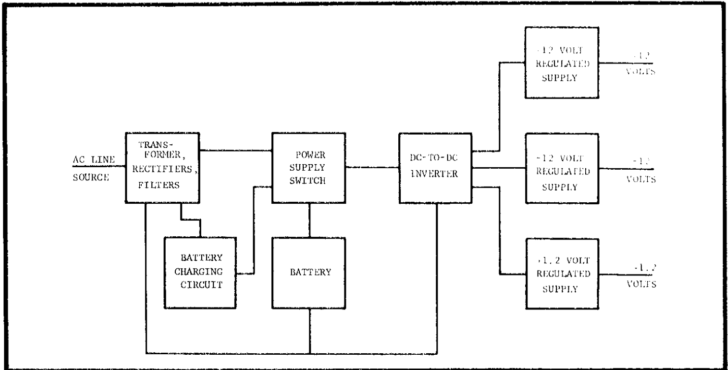
FIGURE 22. Block Diagram of Model 147 Power Supplies and Battery Charging Circuit.
