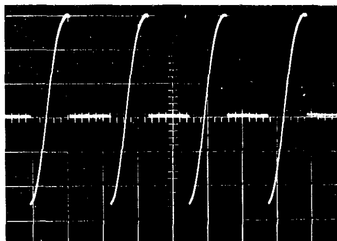
FIGURE 28. Out-of-Phase Wave Form at DEMODULATOR TEST Jack. See paragraph 5-12. Scale is 1 v/cm vertical, 5 msec/cm horizontal.
