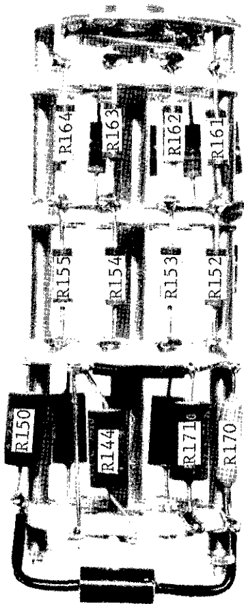
FIGURE 39. Resistor Locations on RANGE Switch (S102). Figure 40 shows resistors on opposite side.
