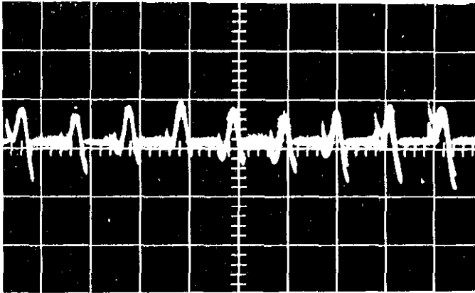
FIGURE 8. Normal Wave Form at Demodulator with Input Shorted. Scale is 0.1 v/cm vertical and 10 msec/cm horizontal.
