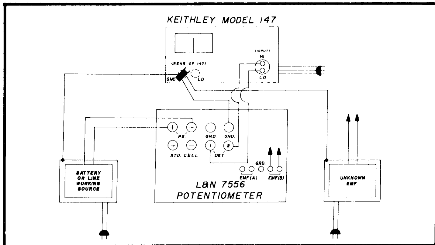
FIGURE 18. Circuit Using Leeds & Northrup 7556 with Keithley Model 147 Null Detector.
