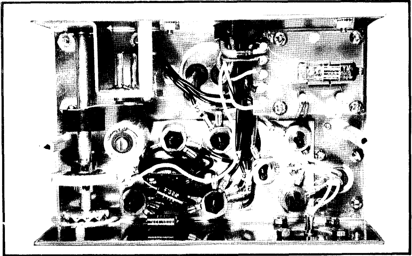
FIGURE 23. Model 147 Input Compartment. Note exact physical location of parts. If replacing, duplicate location and order of leads on posts. Figure 30 gives circuit designations. Refer to Figure 7 for general connection construction.
