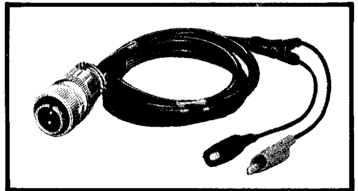
FIGURE 4. Model 1481 Low-Thermal Input Cable. The Model 1482 Low-Thermal Input Cable is similar except it has bare copper leads instead of alligator clips.
