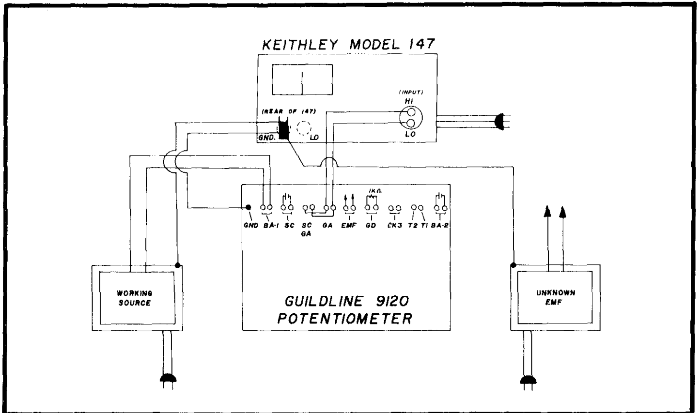
FIGURE 16. Circuit Using Guildline 9120 with Keithley Model 147 Null Detector.
