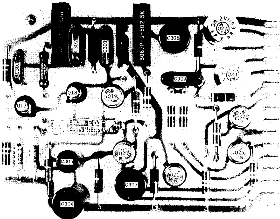
FIGURE 38. Capacitor and Transistor Locations on Printed Circuit 75.
