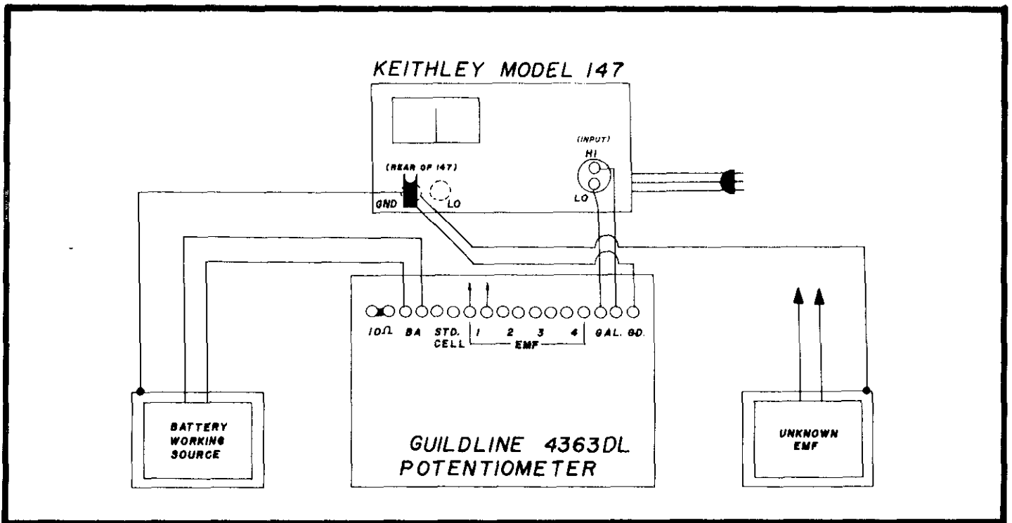
FIGURE 15. Circuit Using Guildline 4363DL with Keithley Model 147 Null Detector.
