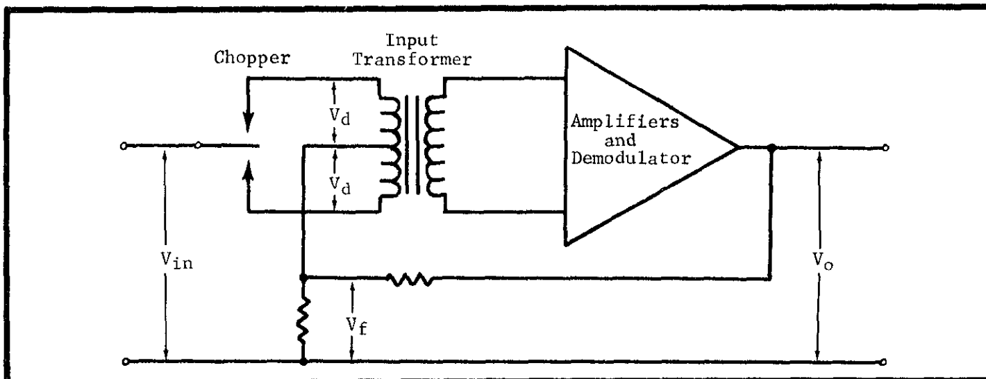
FIGURE 21. Model 147 Input Circuit. The dc input signal, V_{in} , is applied to the chopper. The feedback signal, V_f (the dc amplifier output voltage, V_o , times the feedback ratio, \beta ), is applied to the transformer primary. The signal, V_d , stepped up by the transformer is the difference between the two, V_d = V_{in} - V_f . When the dc input signal is initially applied to the Model 147, V_f is zero and the voltage across the primary is entirely V_{in} . As the output voltage rises, V_f increases and V_d decreases to a small value, then V_f = V_{in} , or \beta V_o = V_{in} . Only \beta , which depends upon the RANGE and FUNCTION Switch settings, determines the amplifier gain.
