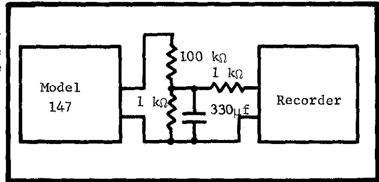
FIGURE 11. 8-cps Filter Circuit for Recorder Output. If the 8-cps beat disturbs the measurements, this circuit will reduce the beat 10:1.
