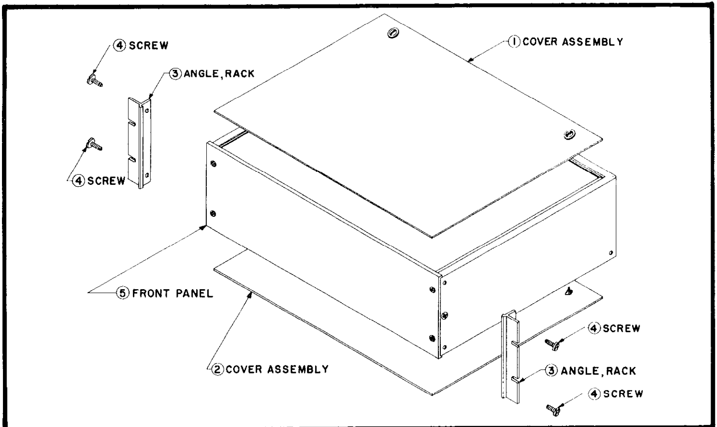
FIGURE 13. Exploded View for Rack Mounting, Using Model 4002 Rack Mounting Kit.
