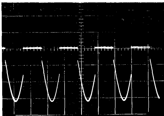
FIGURE 27. Correct Wave Form at DEMODULATOR TEST Jack. See paragraph 5-12. Scale is 1 v/cm vertical, 5 msec/cm horizontal.
