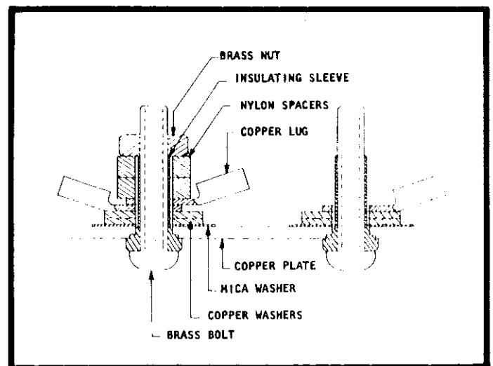
FIGURE 7. Thermal Sink Construction. Connect leads or lugs as close as possible. Separate only with insulation of high heat conductivity.
