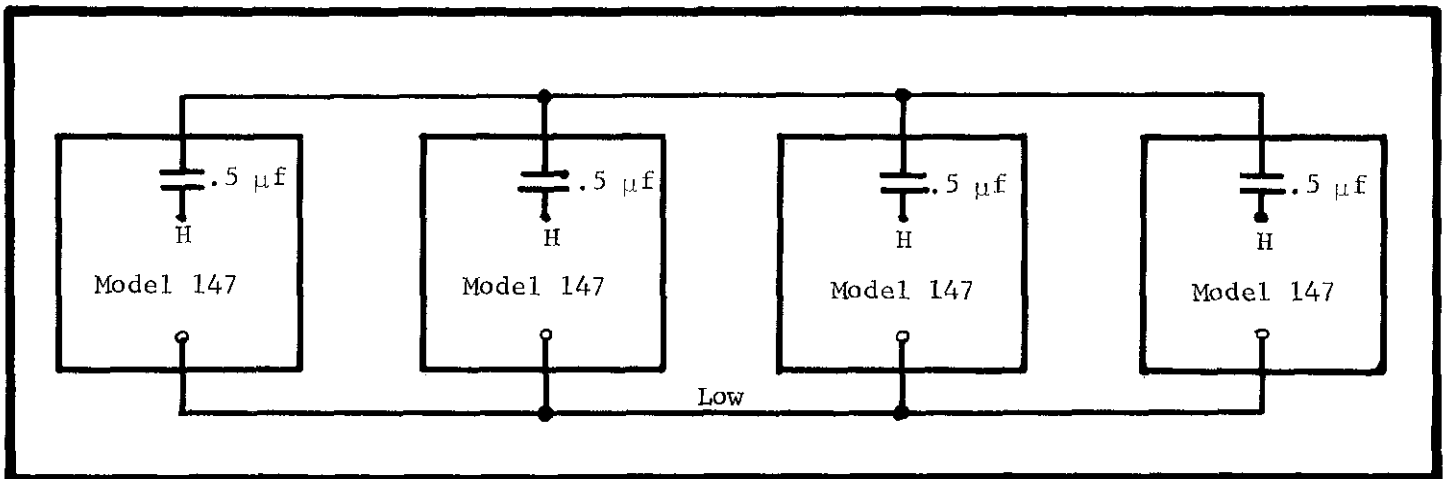
FIGURE 6. Synchronized Buss System for Model 147. When two or more Null Detectors are used in one system, an oscillator beat may occur; see paragraph 2-10. Synchronize the instruments by connecting them as shown. See Figure 29 for point H.
