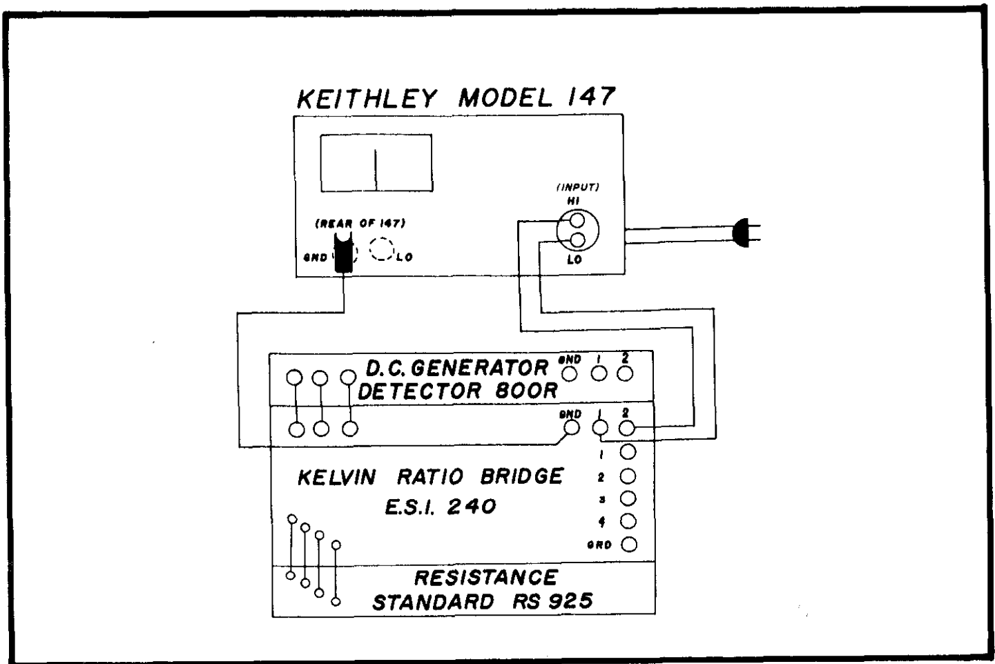
FIGURE 19. Circuit Using Keithley Model 147 Null Detector with ESI 240, 800R and RS 925.
