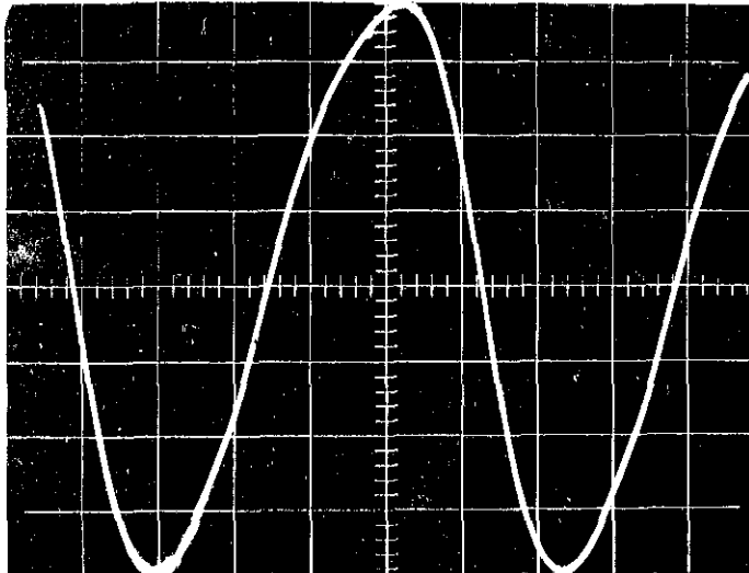
FIGURE 25. Correct Wave Form at Point F (Figure 30) in Oscillator Circuit. Scale is 2 v/cm vertical, 2 msec/cm horizontal.
