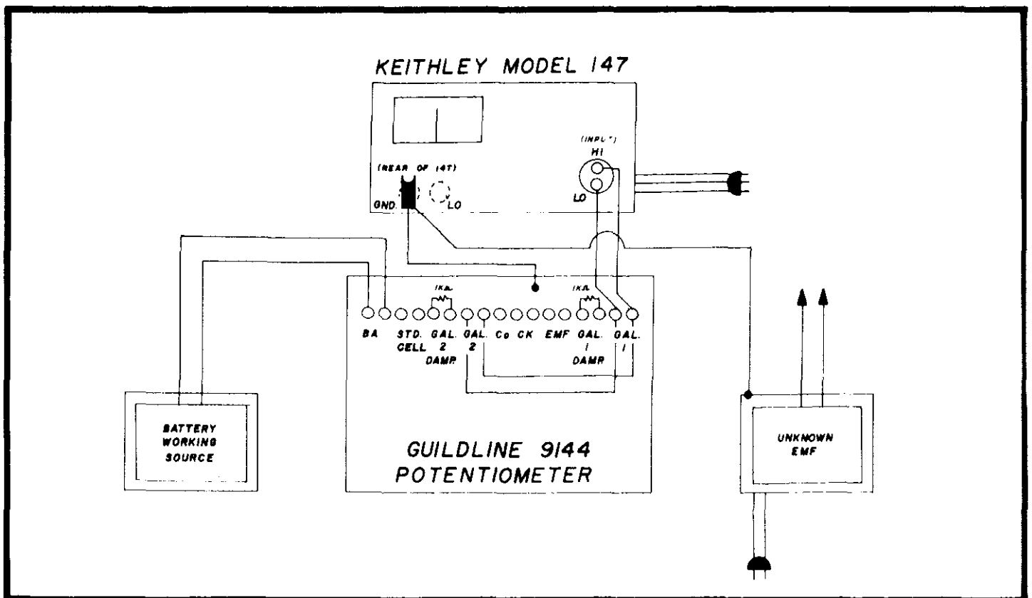
FIGURE 14. Circuit Using Guildline 9144 with Keithley Model 147 Null Detector.
