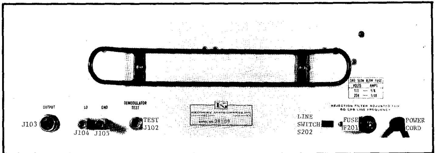
FIGURE 3. Model 147 Rear Panel Controls and Connections. Circuit designations refer to Replaceable Parts List and schematic diagrams.
