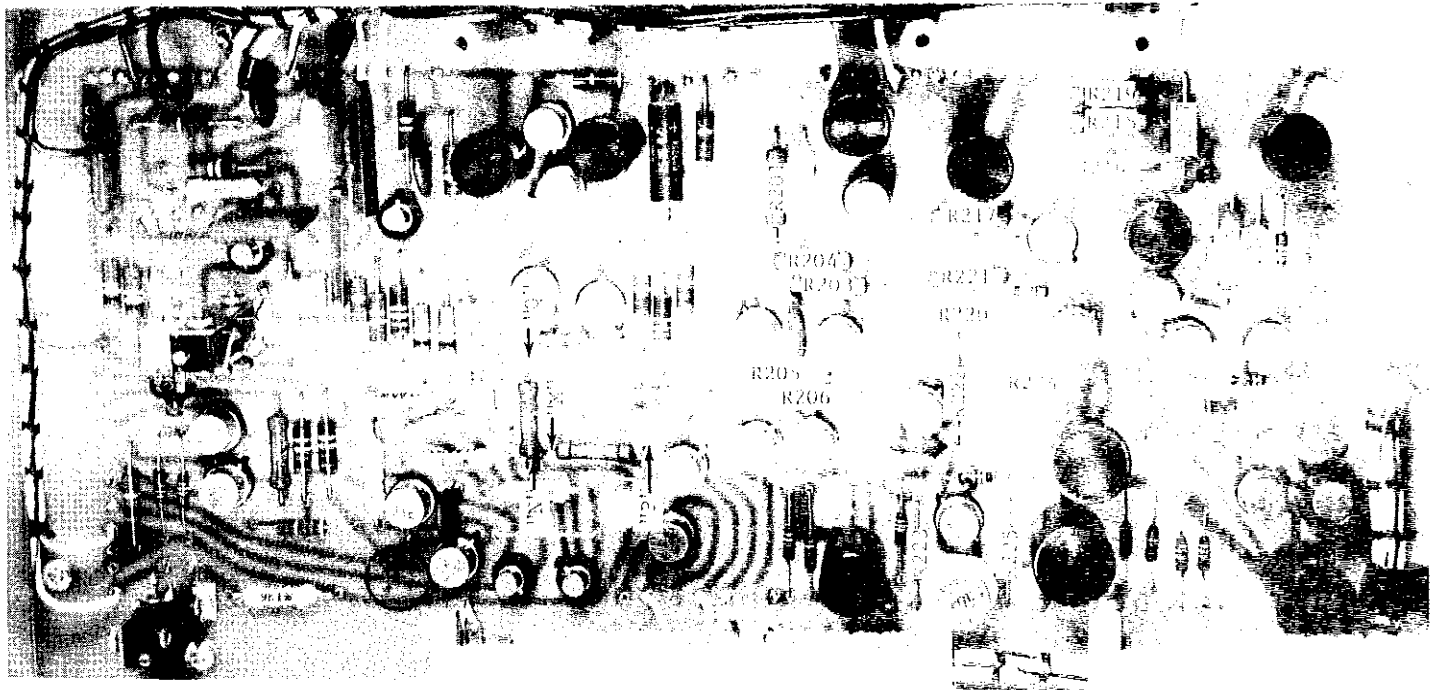
FIGURE 34. Resistor and Test Point Locations on Printed Circuit 76. Figure 33 contains callouts for the other resistors
