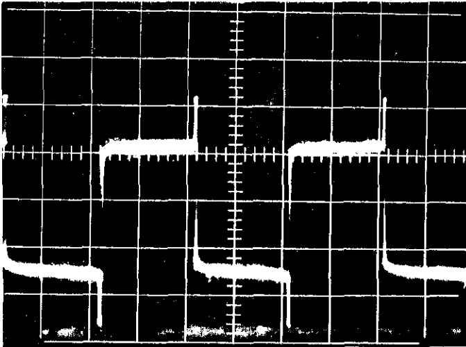
FIGURE 24. Correct Wave Form in dc-to-dc Inverter. Point E, Figure 35, was monitored. Scale is 5 v/cm vertical, 0.2 msec/cm horizontal.
