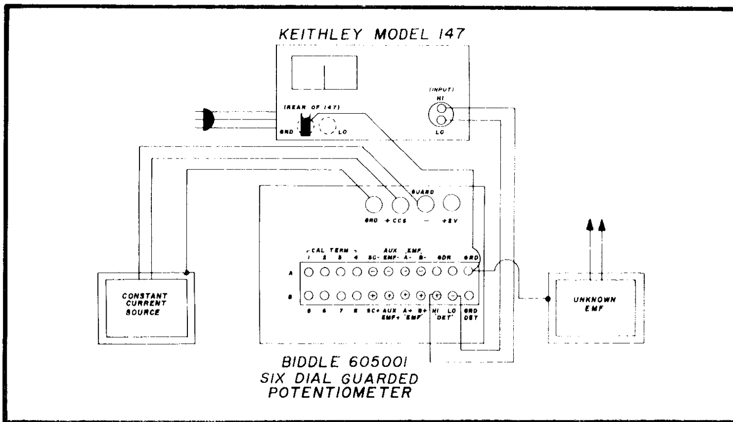
FIGURE 17. Circuit Using Biddle 605001 with Keithley Model 147 Null Detector.
